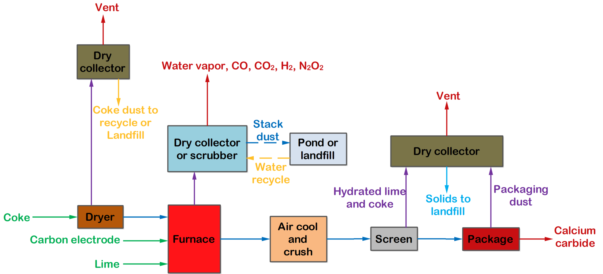
Figure: Manufacture of Calcium carbide by open furnace
